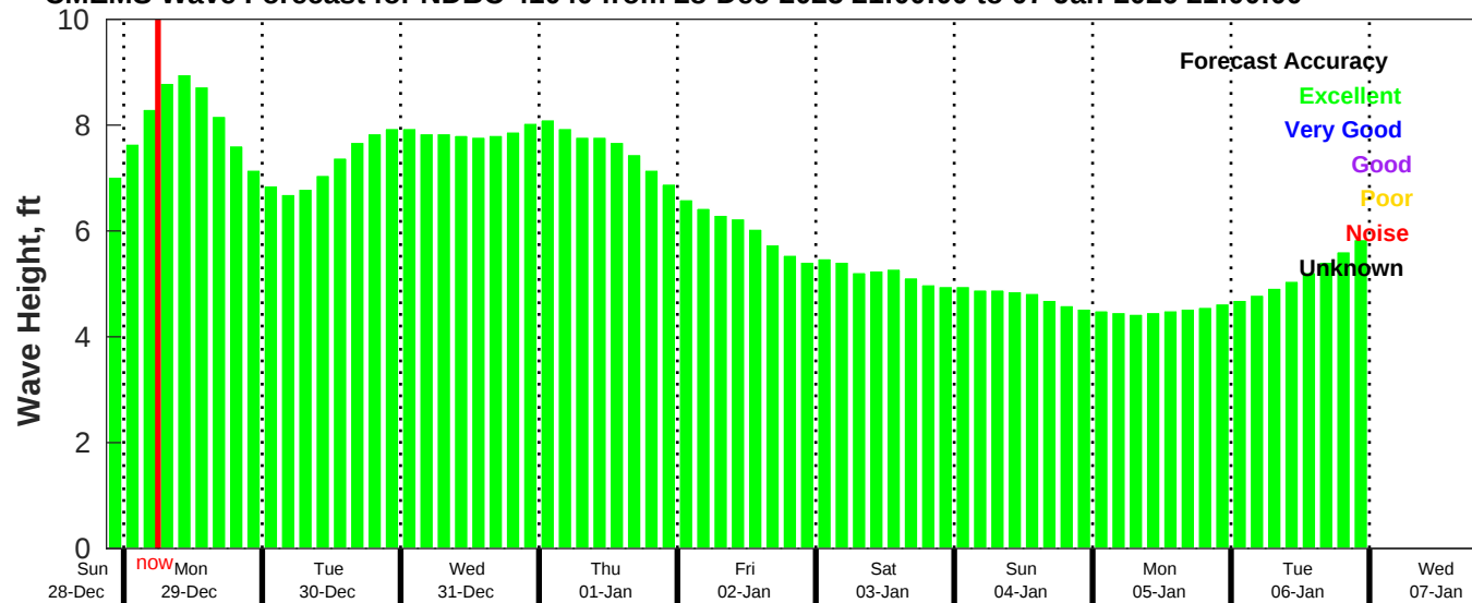
CMEMS Wave Forecast for NDBC 41040 from 28-Dec-2025 21:00:00 to 07-Jan-2026 21:00:00
