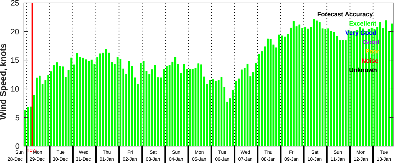
GFS Wind Speed Forecast for NDBC 41040 from 28-Dec-2025 21:00:00 to 13-Jan-2026 21:00:00
