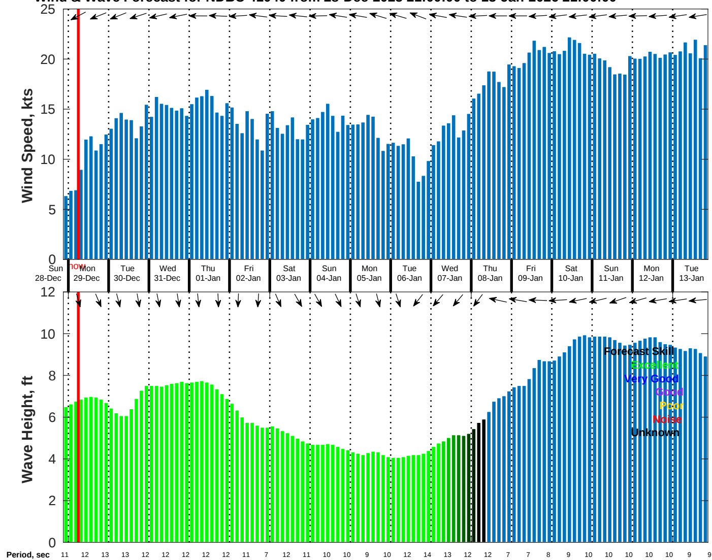
Wind & Wave Forecast for NDBC 41040 from 28-Dec-2025 21:00:00 to 13-Jan-2026 21:00:00
