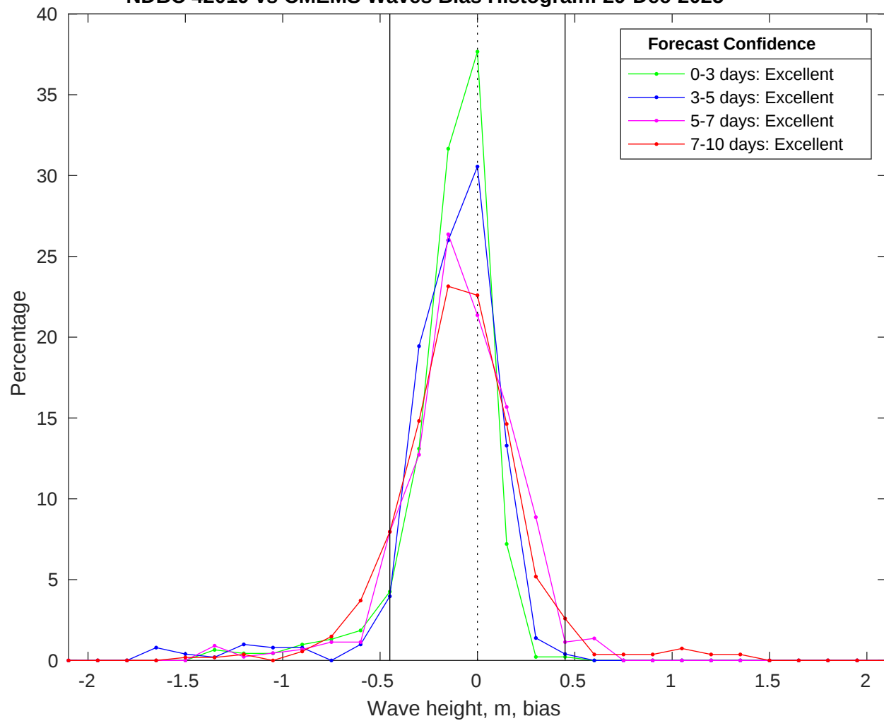
NDBC 42019 vs CMEMS Waves Bias Histogram: 29-Dec-2025
