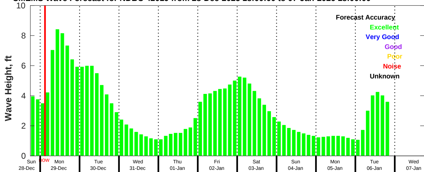
CMEMS Wave Forecast for NDBC 42019 from 28-Dec-2025 18:00:00 to 07-Jan-2026 18:00:00
