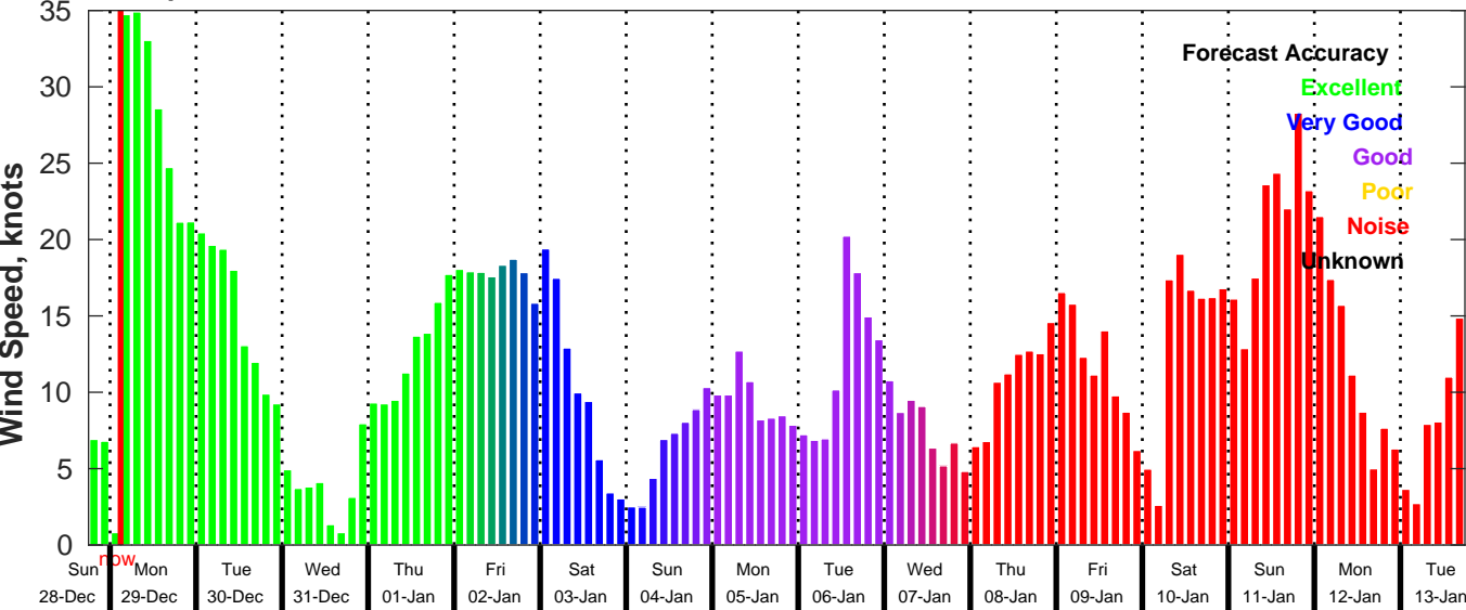
GFS Wind Speed Forecast for NDBC 42019 from 28-Dec-2025 18:00:00 to 13-Jan-2026 18:00:00
