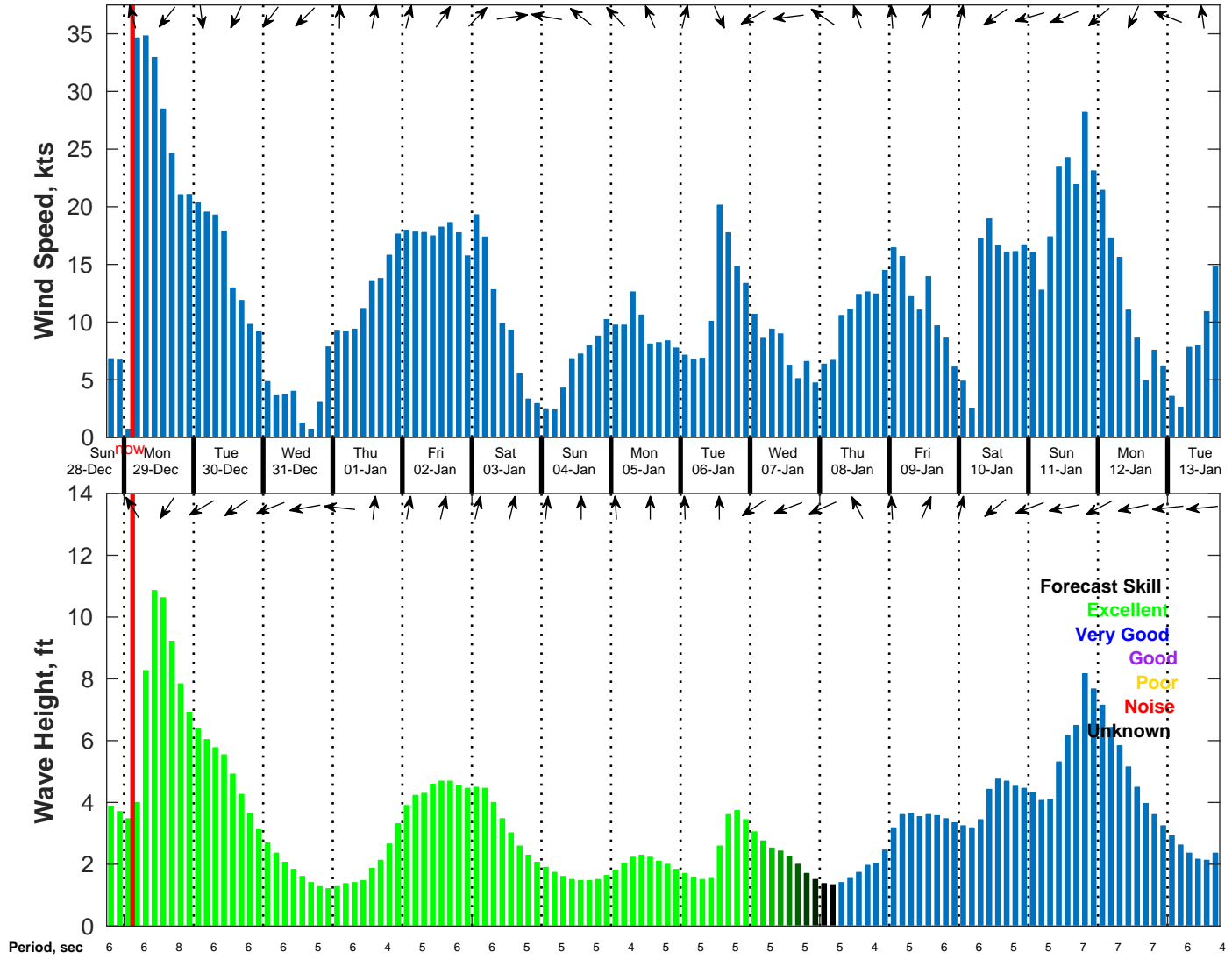
Wind & Wave Forecast for NDBC 42019 from 28-Dec-2025 18:00:00 to 13-Jan-2026 18:00:00
