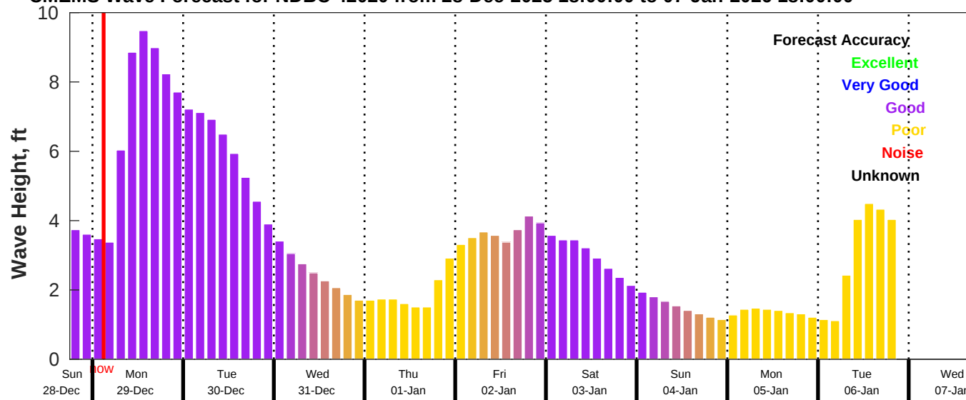
CMEMS Wave Forecast for NDBC 42020 from 28-Dec-2025 18:00:00 to 07-Jan-2026 18:00:00
