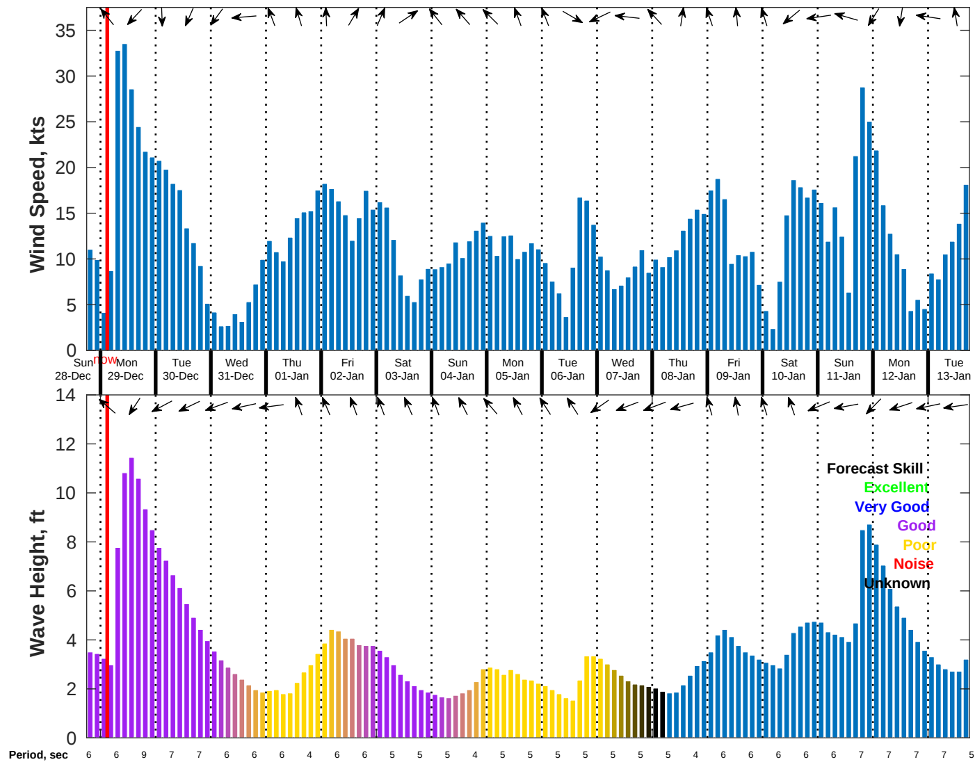
Wind & Wave Forecast for NDBC 42020 from 28-Dec-2025 18:00:00 to 13-Jan-2026 18:00:00
