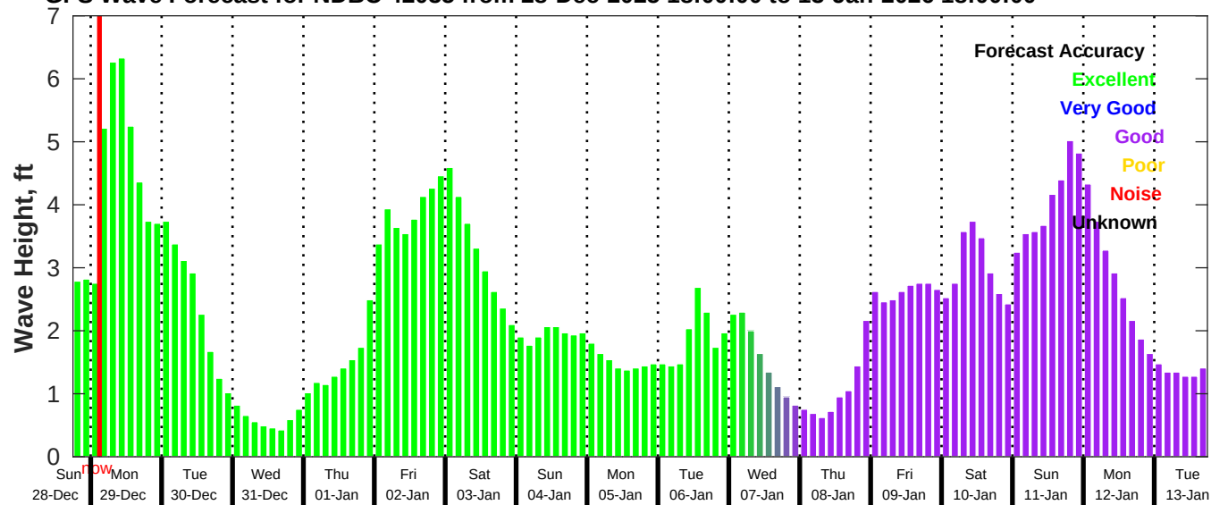
GFS Wave Forecast for NDBC 42035 from 28-Dec-2025 18:00:00 to 13-Jan-2026 18:00:00
