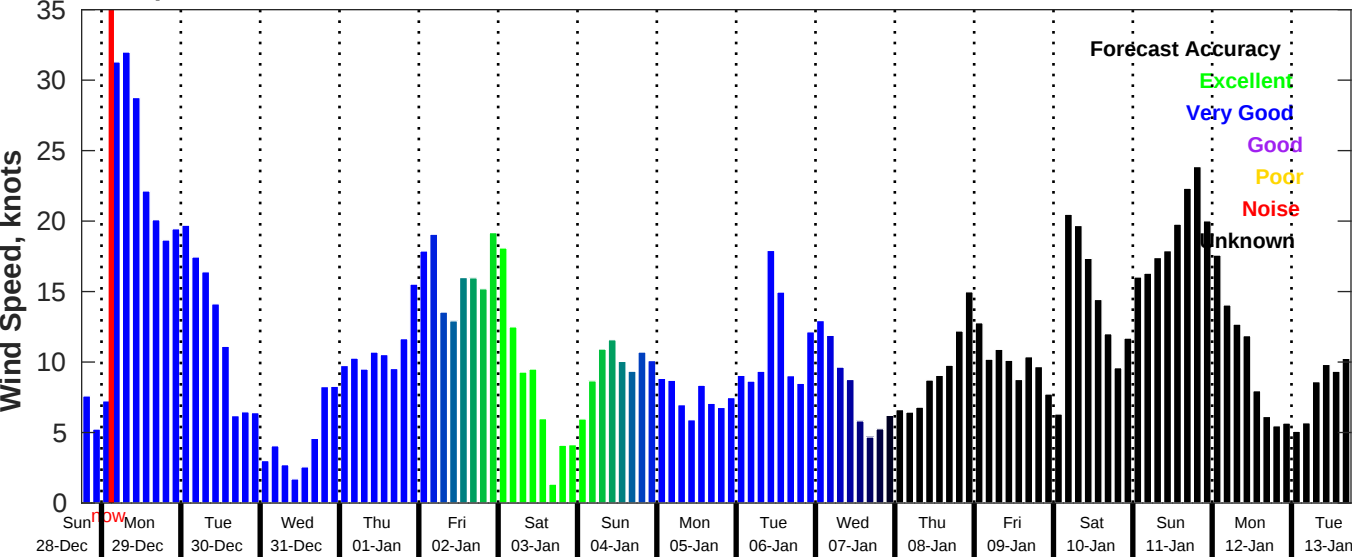
GFS Wind Speed Forecast for NDBC 42035 from 28-Dec-2025 18:00:00 to 13-Jan-2026 18:00:00
