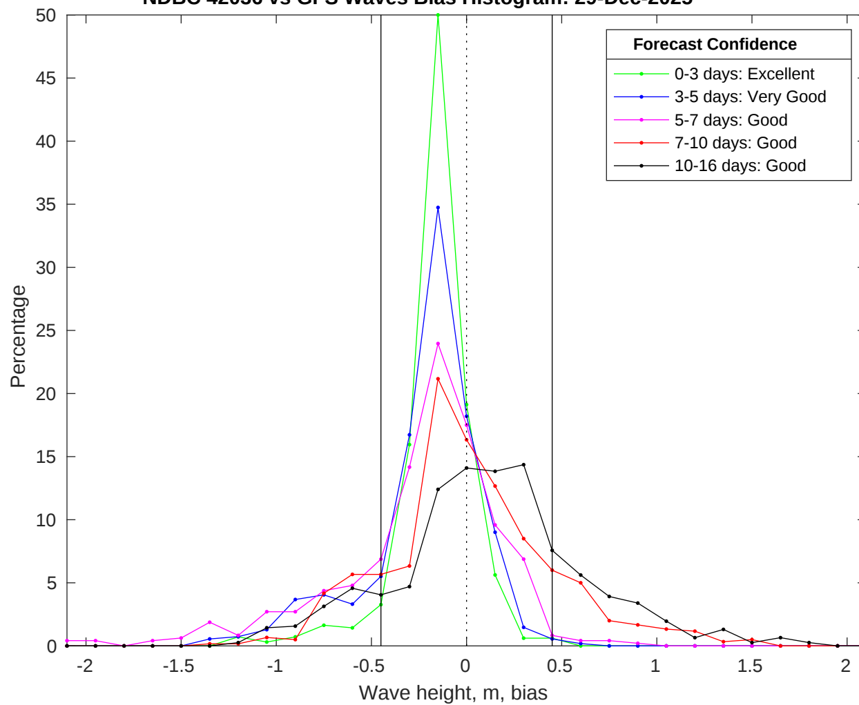
NDBC 42036 vs GFS Waves Bias Histogram: 29-Dec-2025
