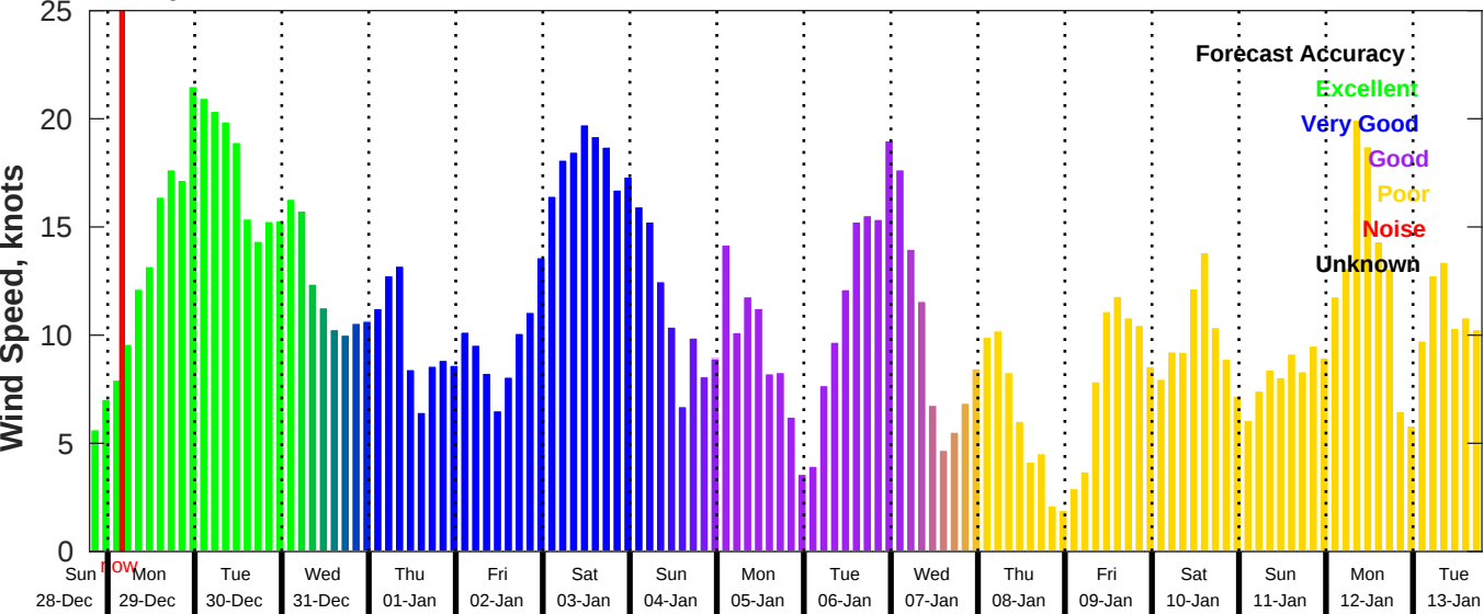
GFS Wind Speed Forecast for NDBC 42036 from 28-Dec-2025 19:00:00 to 13-Jan-2026 19:00:00
