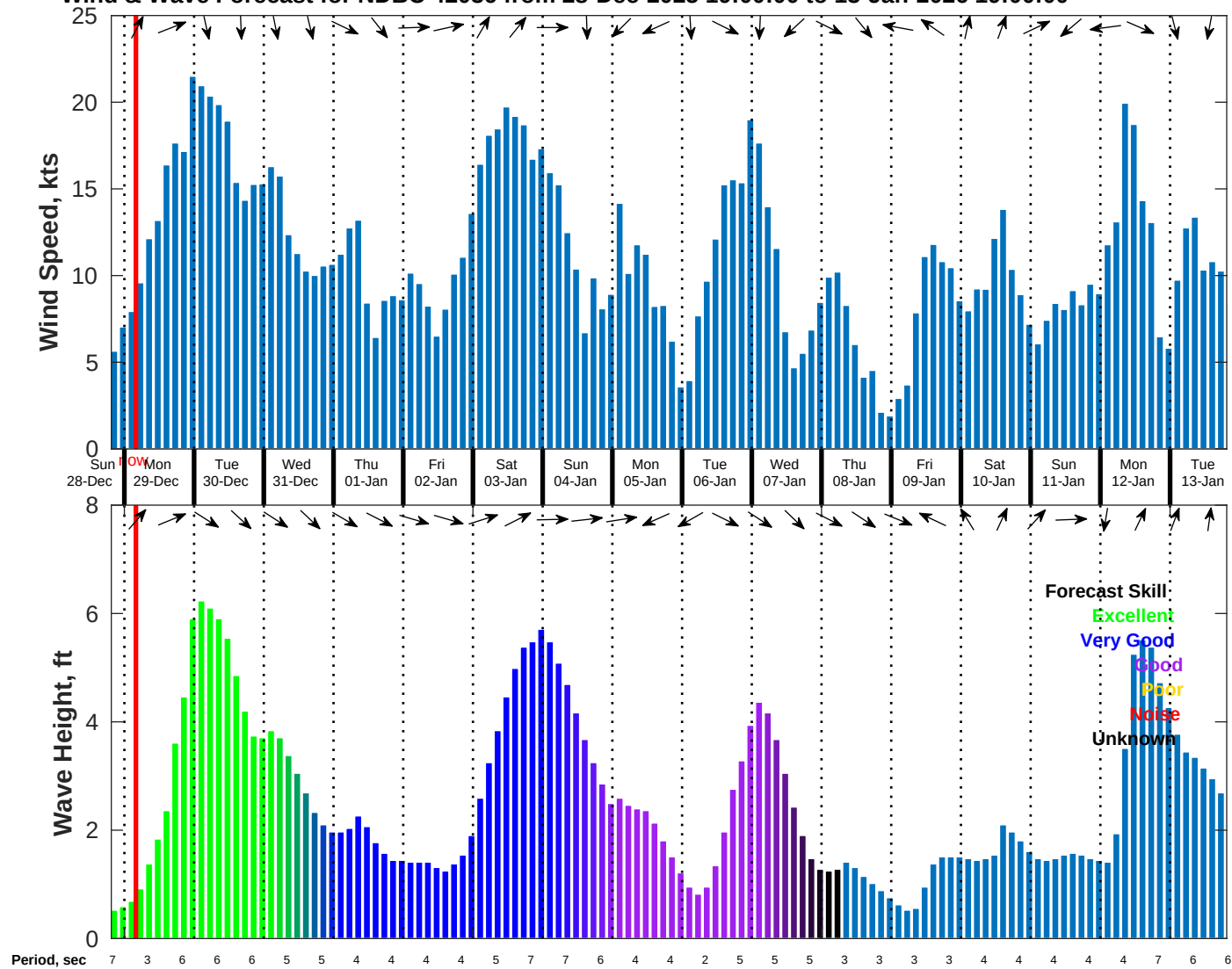
Wind & Wave Forecast for NDBC 42036 from 28-Dec-2025 19:00:00 to 13-Jan-2026 19:00:00
