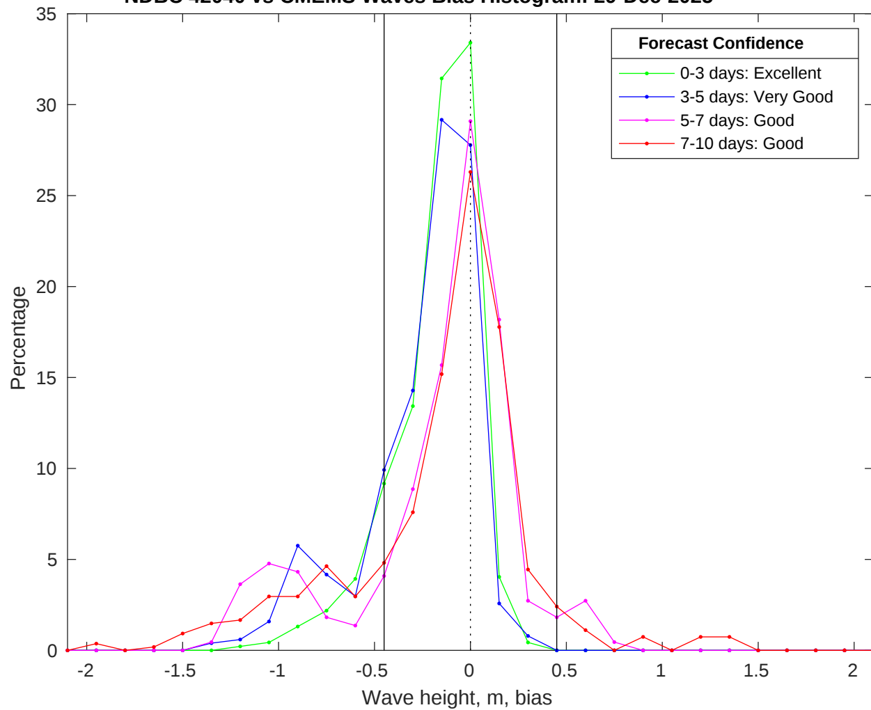
NDBC 42040 vs CMEMS Waves Bias Histogram: 29-Dec-2025
