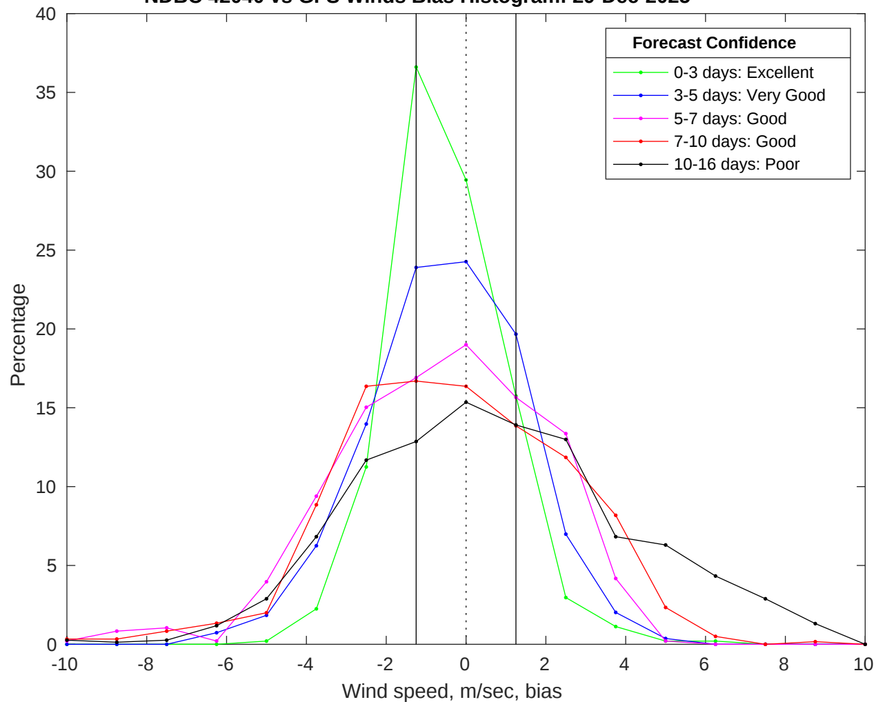
NDBC 42040 vs GFS Winds Bias Histogram: 29-Dec-2025
