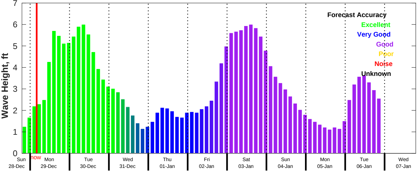
CMEMS Wave Forecast for NDBC 42040 from 28-Dec-2025 19:00:00 to 07-Jan-2026 19:00:00
