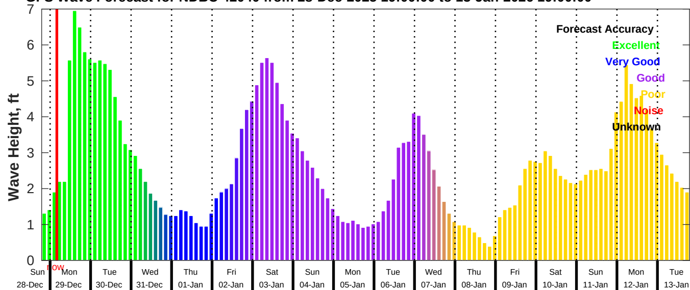
GFS Wave Forecast for NDBC 42040 from 28-Dec-2025 19:00:00 to 13-Jan-2026 19:00:00
