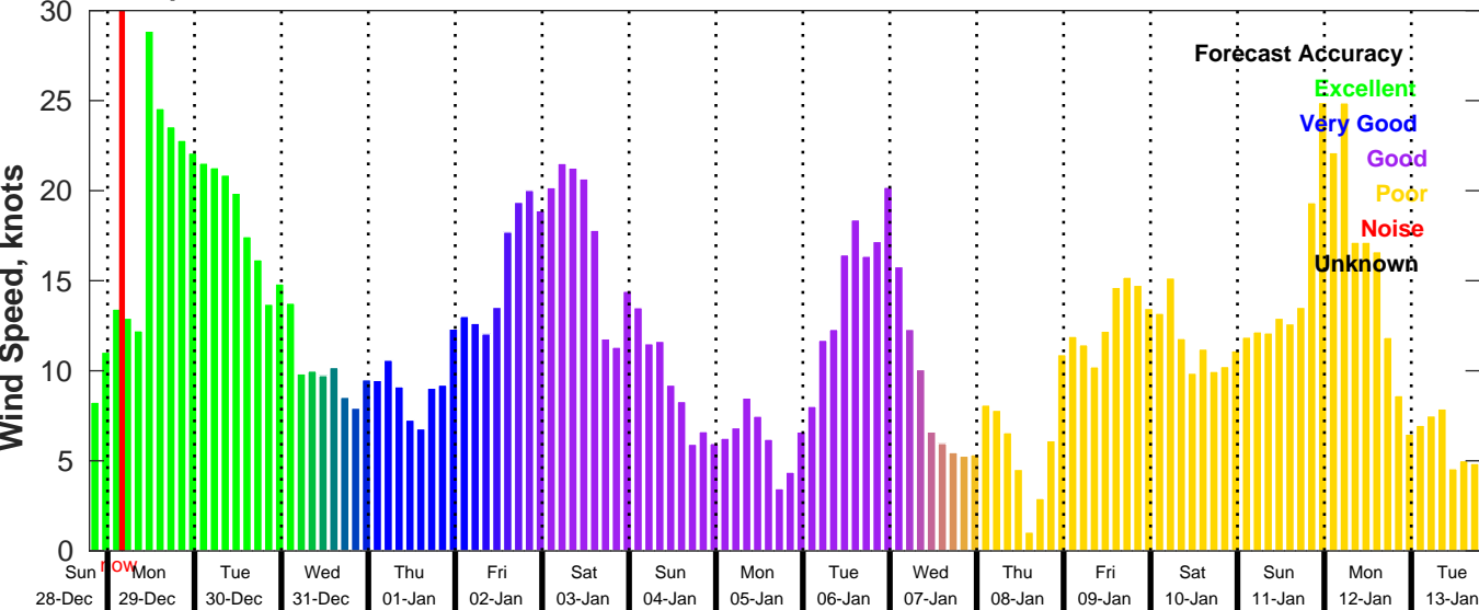
GFS Wind Speed Forecast for NDBC 42040 from 28-Dec-2025 19:00:00 to 13-Jan-2026 19:00:00
