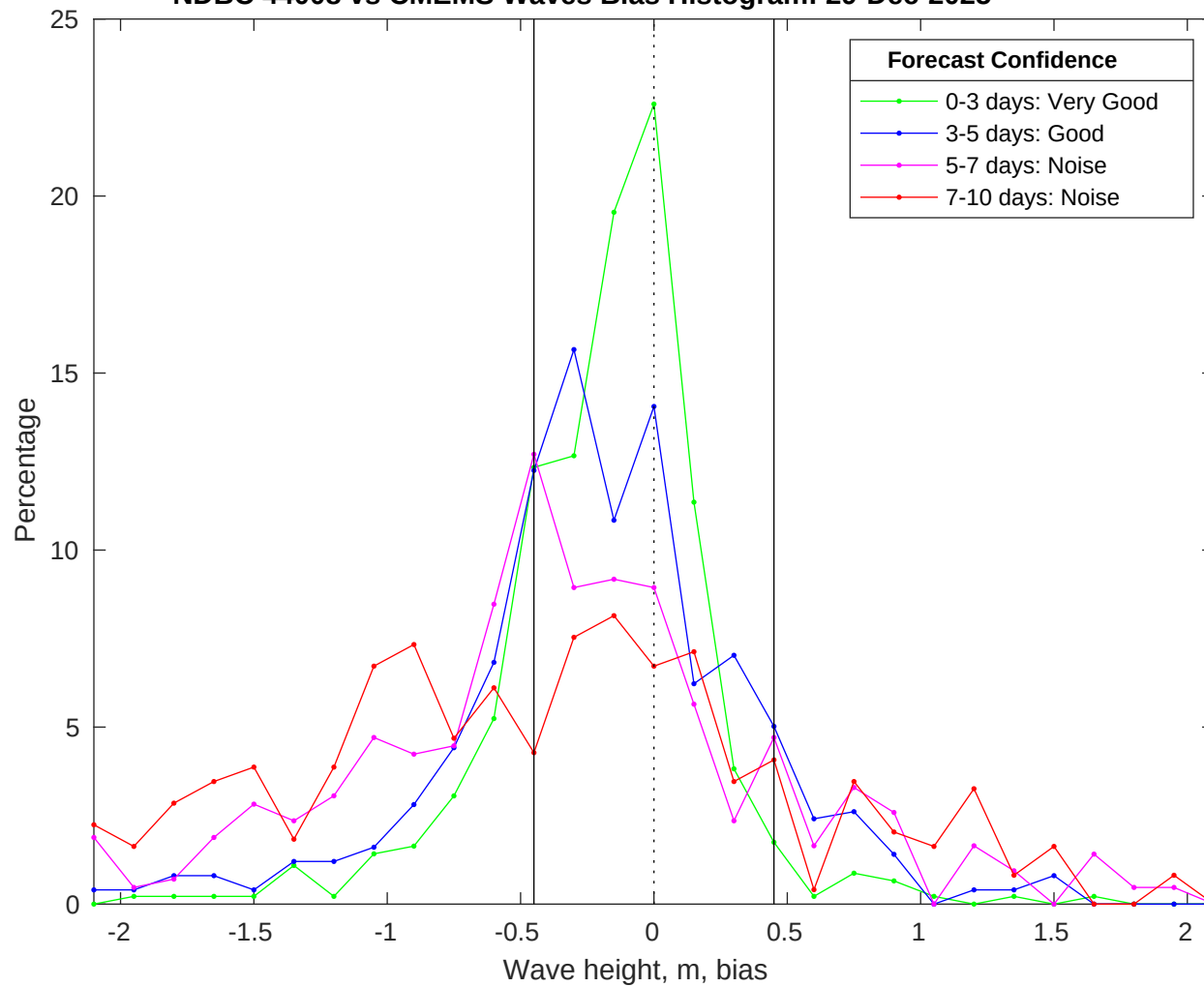
NDBC 44008 vs CMEMS Waves Bias Histogram: 29-Dec-2025
