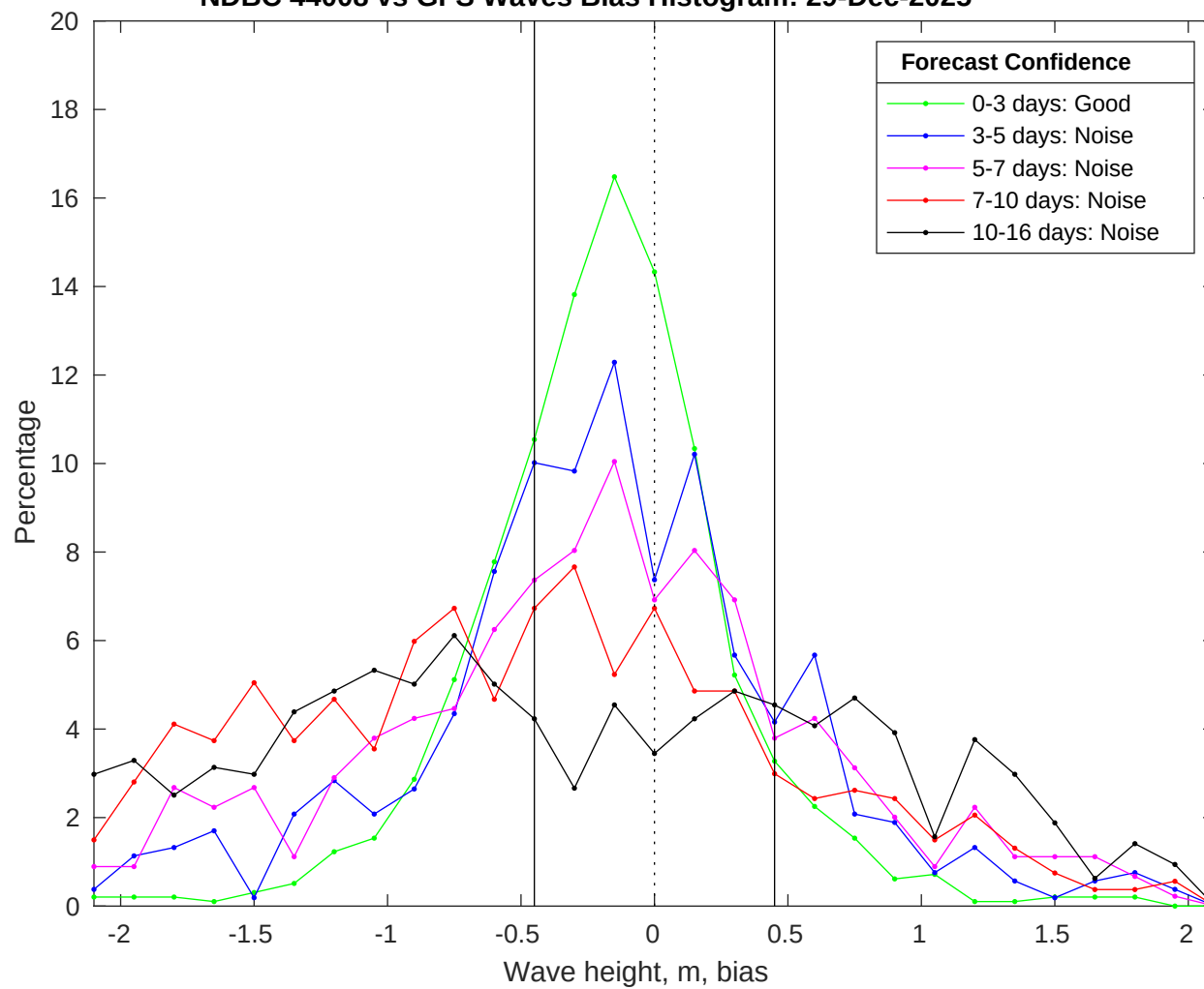
NDBC 44008 vs GFS Waves Bias Histogram: 29-Dec-2025
