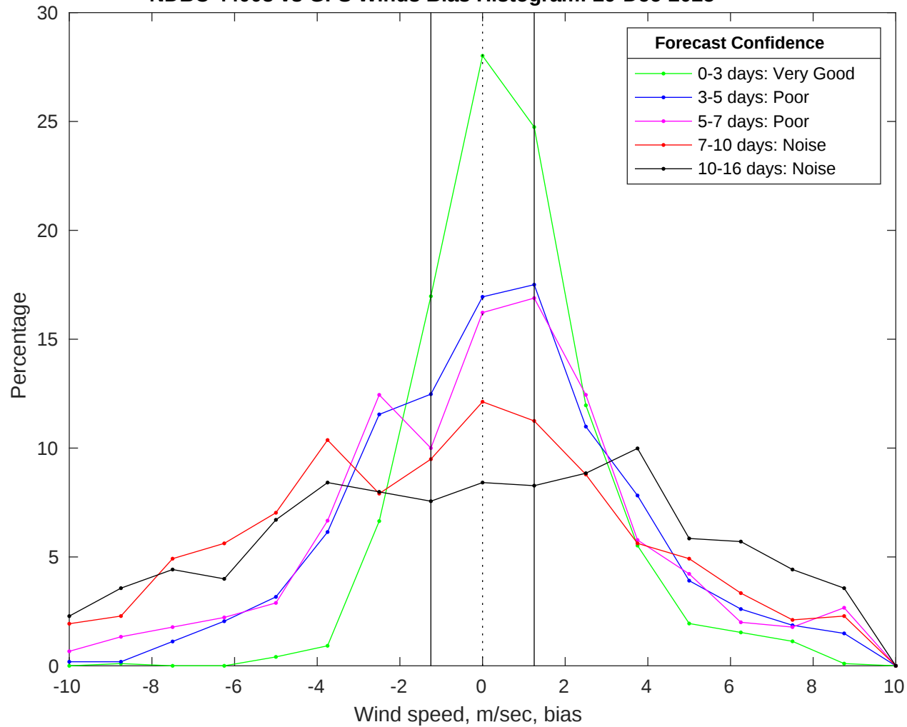
NDBC 44008 vs GFS Winds Bias Histogram: 29-Dec-2025
