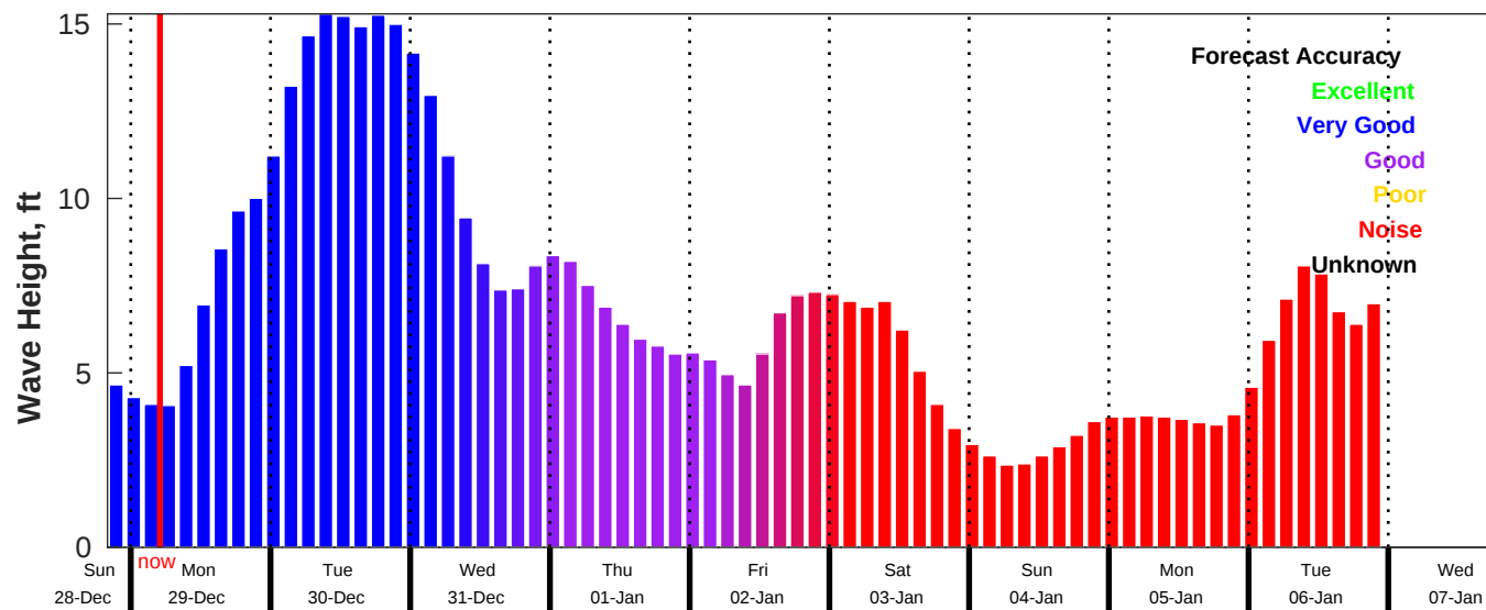
CMEMS Wave Forecast for NDBC 44008 from 28-Dec-2025 20:00:00 to 07-Jan-2026 20:00:00
