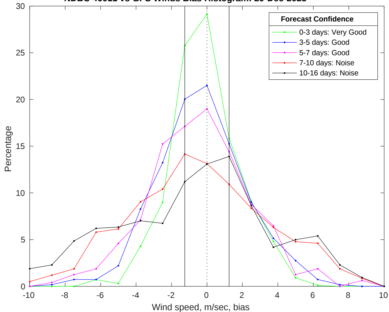
NDBC 46011 vs GFS Winds Bias Histogram: 29-Dec-2025
