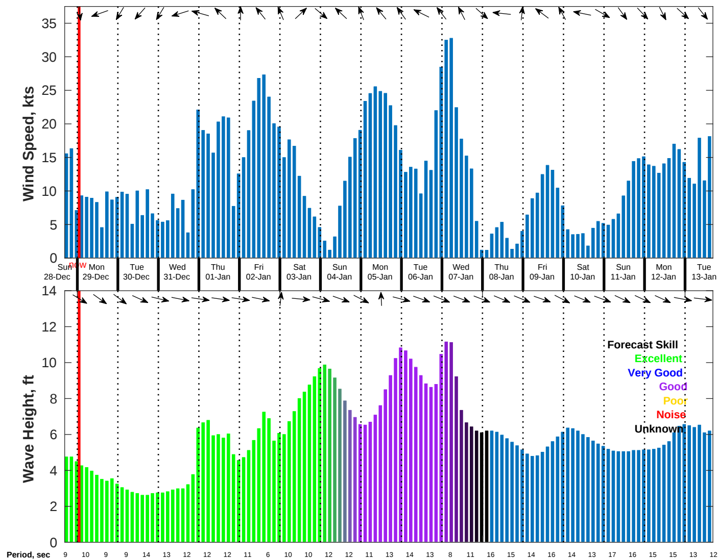
Wind & Wave Forecast for NDBC 46011 from 28-Dec-2025 16:00:00 to 13-Jan-2026 16:00:00
