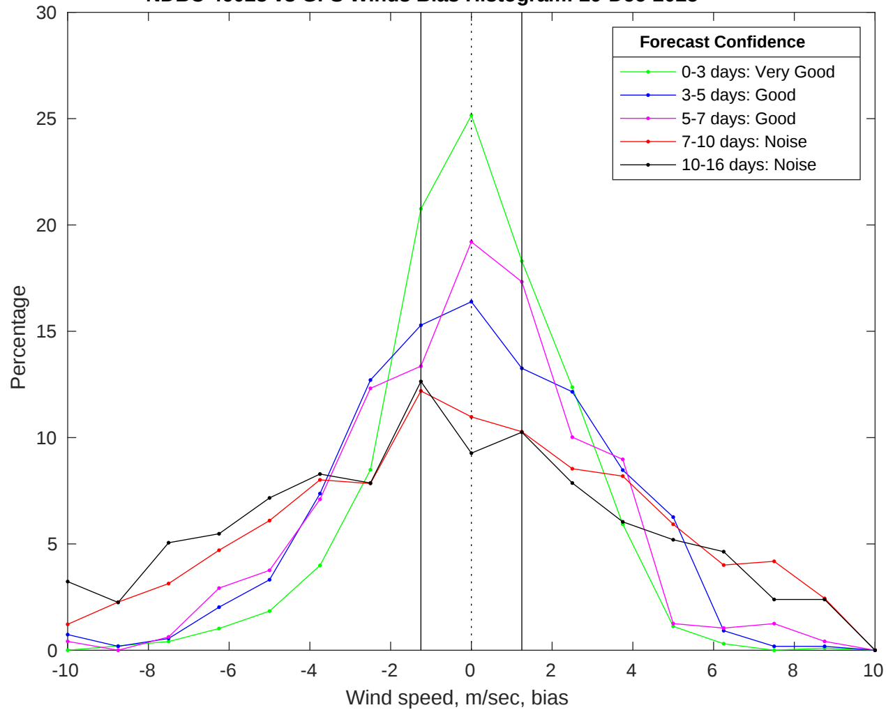
NDBC 46028 vs GFS Winds Bias Histogram: 29-Dec-2025
