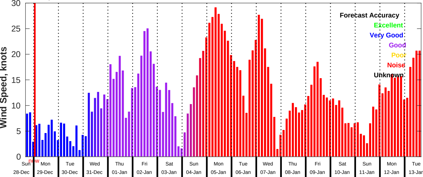
GFS Wind Speed Forecast for NDBC 46028 from 28-Dec-2025 16:00:00 to 13-Jan-2026 16:00:00
