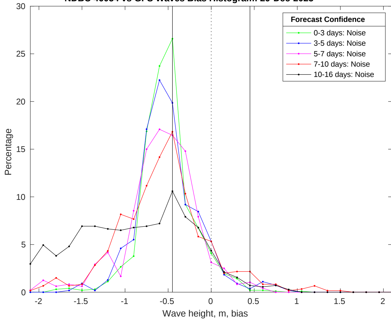
NDBC 46054 vs GFS Waves Bias Histogram: 29-Dec-2025
