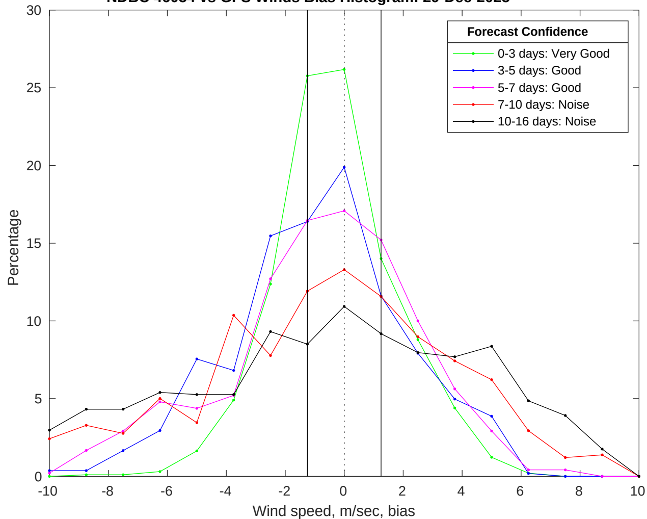
NDBC 46054 vs GFS Winds Bias Histogram: 29-Dec-2025
