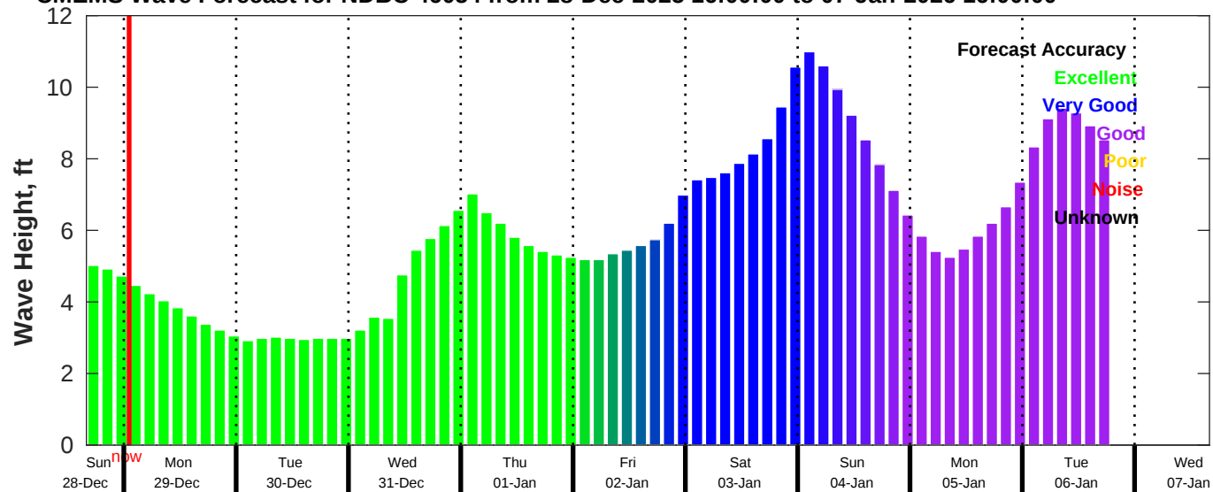
CMEMS Wave Forecast for NDBC 46054 from 28-Dec-2025 16:00:00 to 07-Jan-2026 16:00:00
