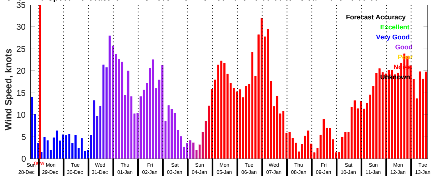
GFS Wind Speed Forecast for NDBC 46054 from 28-Dec-2025 16:00:00 to 13-Jan-2026 16:00:00
