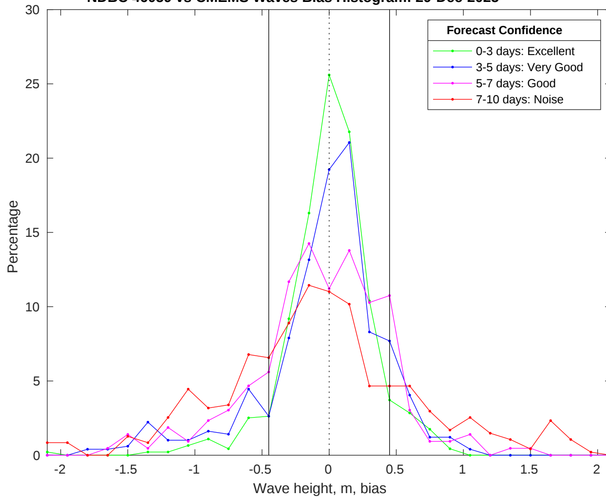
NDBC 46059 vs CMEMS Waves Bias Histogram: 29-Dec-2025
