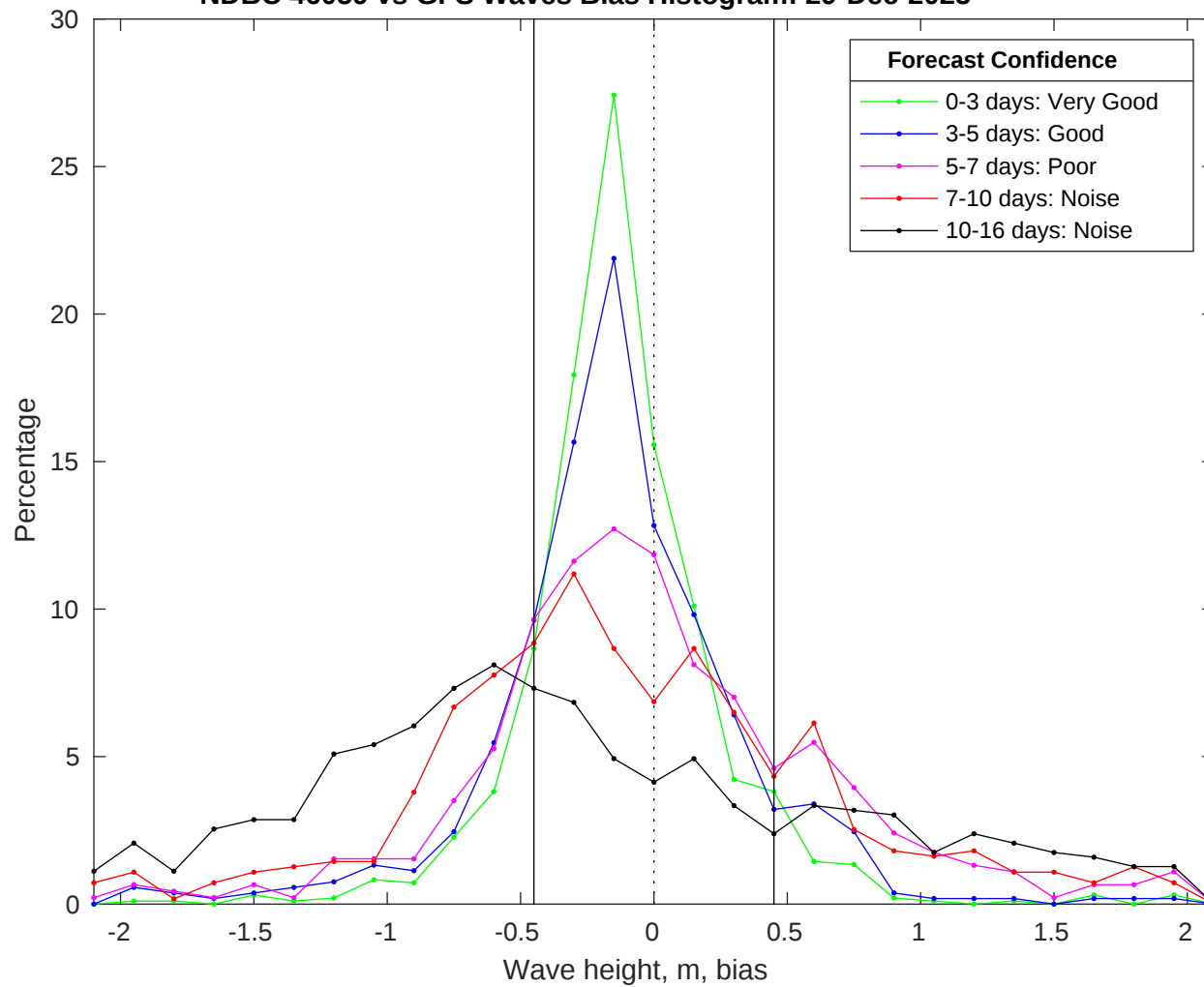
NDBC 46059 vs GFS Waves Bias Histogram: 29-Dec-2025
