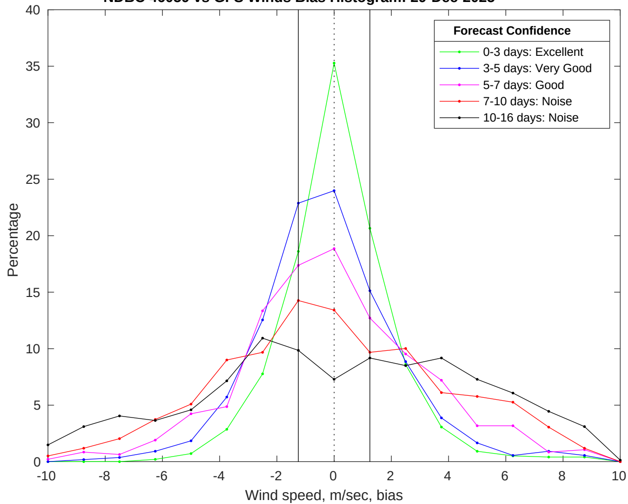
NDBC 46059 vs GFS Winds Bias Histogram: 29-Dec-2025
