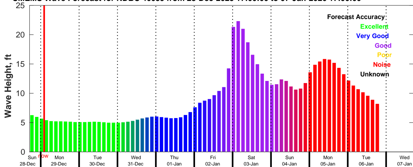
CMEMS Wave Forecast for NDBC 46059 from 28-Dec-2025 17:00:00 to 07-Jan-2026 17:00:00
