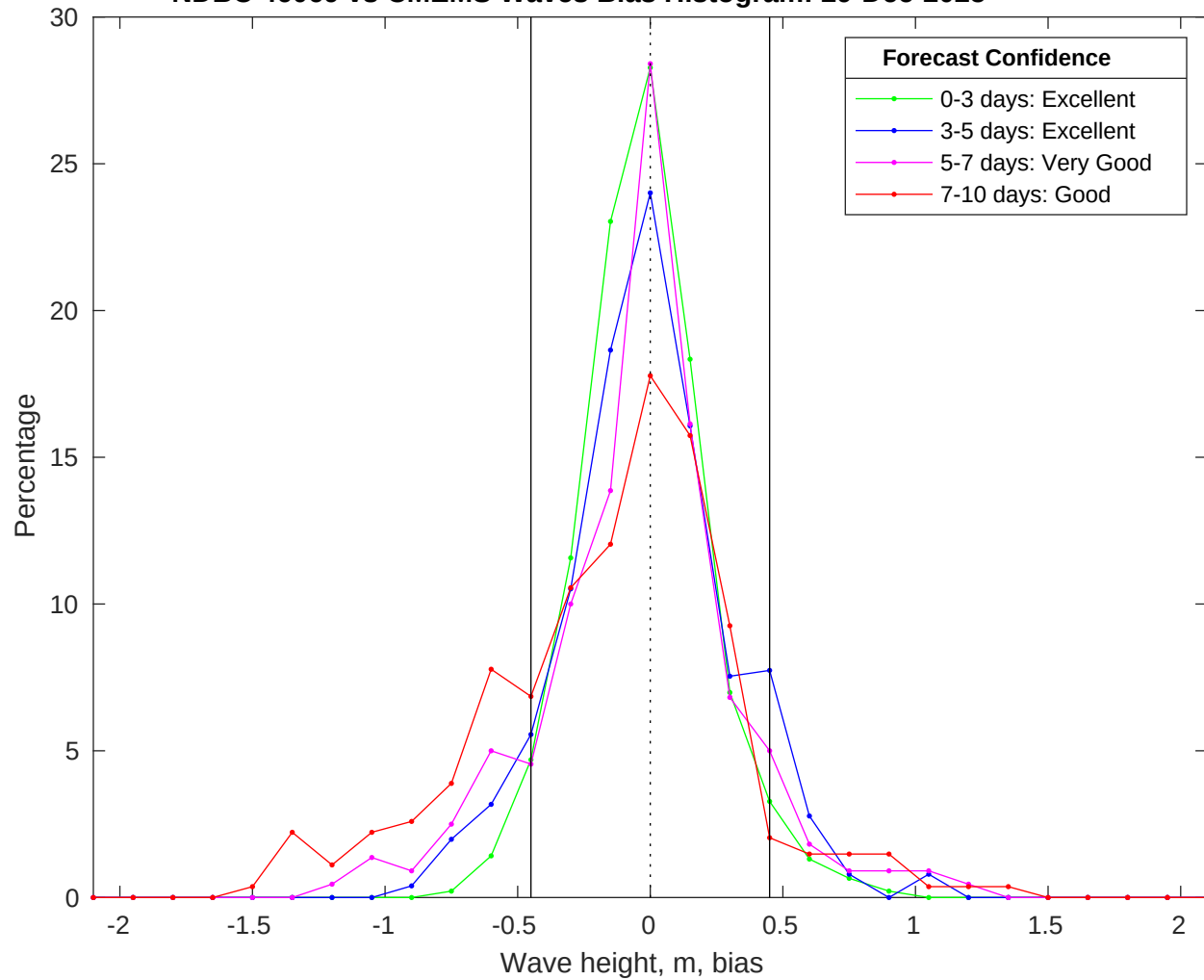
NDBC 46069 vs CMEMS Waves Bias Histogram: 29-Dec-2025
