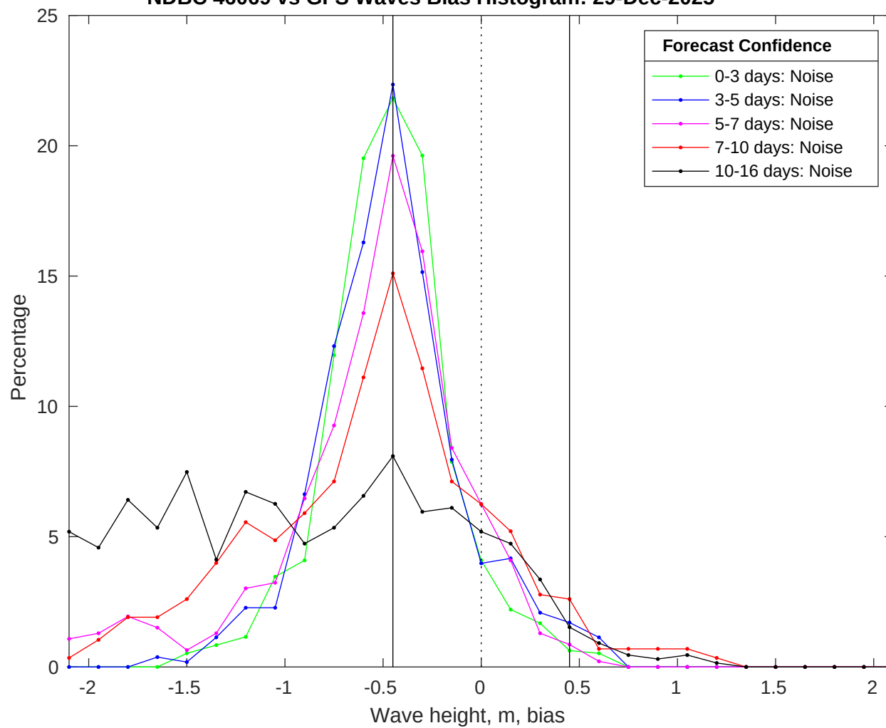
NDBC 46069 vs GFS Waves Bias Histogram: 29-Dec-2025
