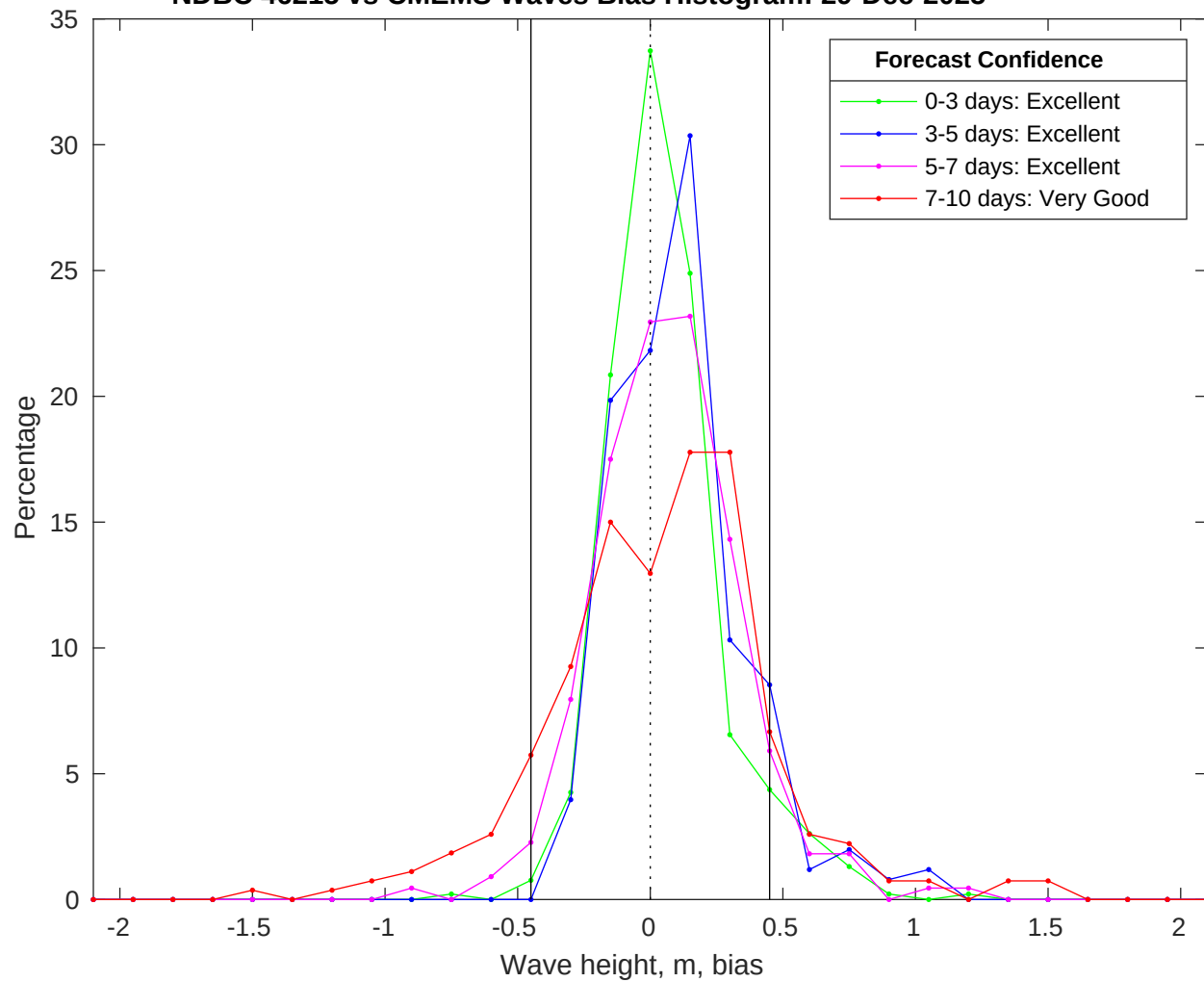
NDBC 46215 vs CMEMS Waves Bias Histogram: 29-Dec-2025
