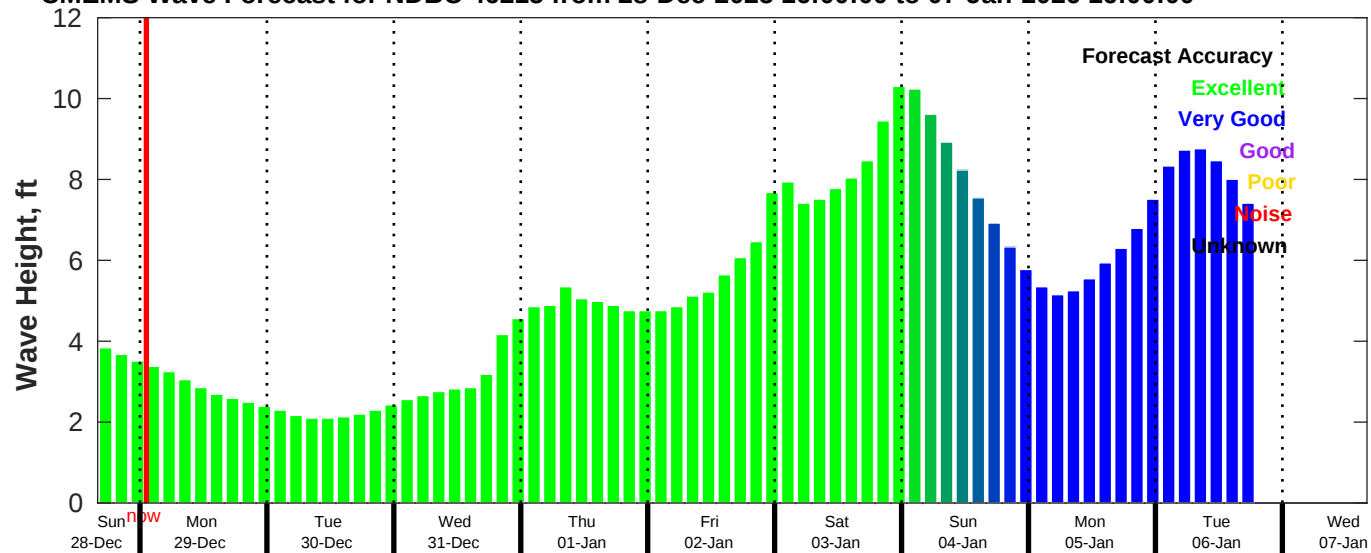
CMEMS Wave Forecast for NDBC 46215 from 28-Dec-2025 16:00:00 to 07-Jan-2026 16:00:00
