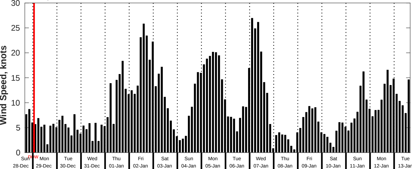
GFS Wind Speed Forecast for NDBC 46215 from 28-Dec-2025 16:00:00 to 13-Jan-2026 16:00:00
