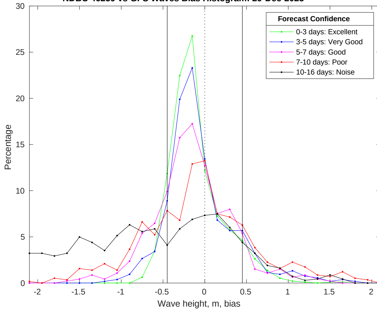
NDBC 46259 vs GFS Waves Bias Histogram: 29-Dec-2025
