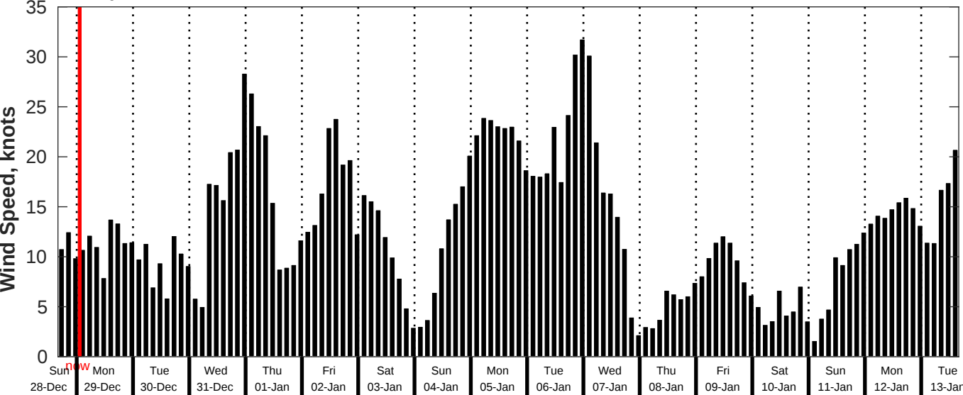
GFS Wind Speed Forecast for NDBC 46259 from 28-Dec-2025 16:00:00 to 13-Jan-2026 16:00:00
