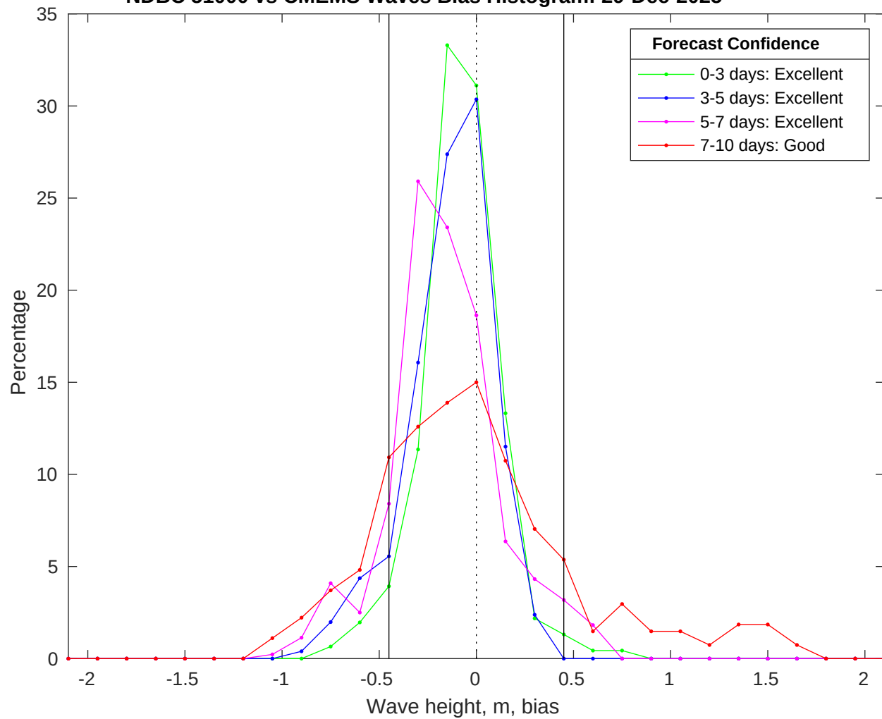
NDBC 51000 vs CMEMS Waves Bias Histogram: 29-Dec-2025
