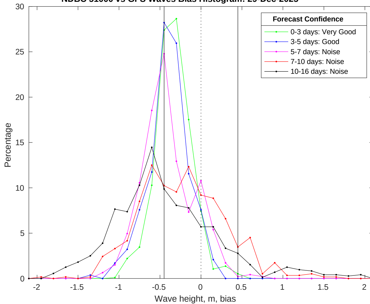
NDBC 51000 vs GFS Waves Bias Histogram: 29-Dec-2025
