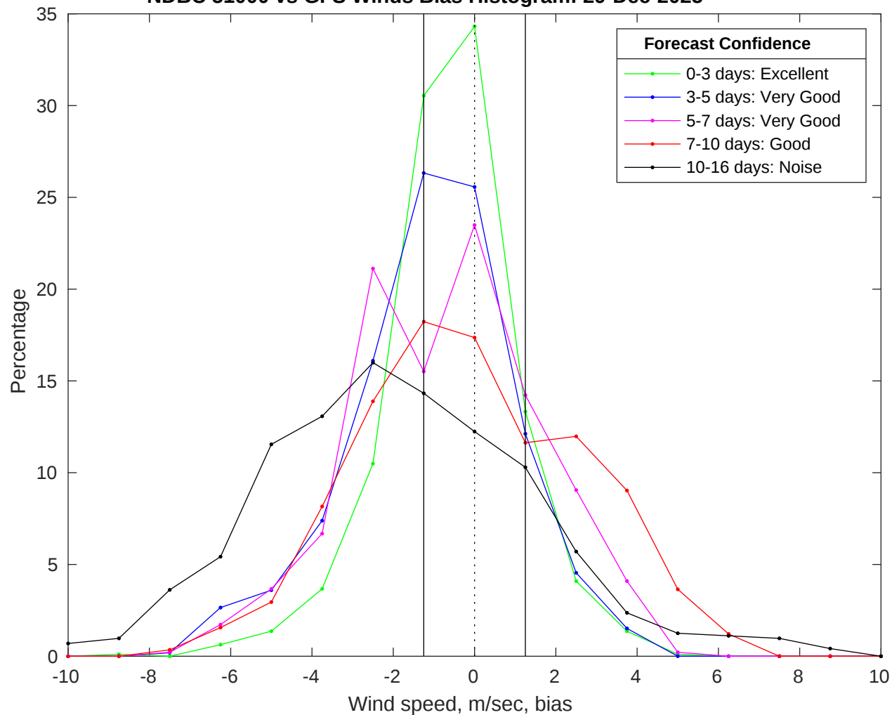
NDBC 51000 vs GFS Winds Bias Histogram: 29-Dec-2025
