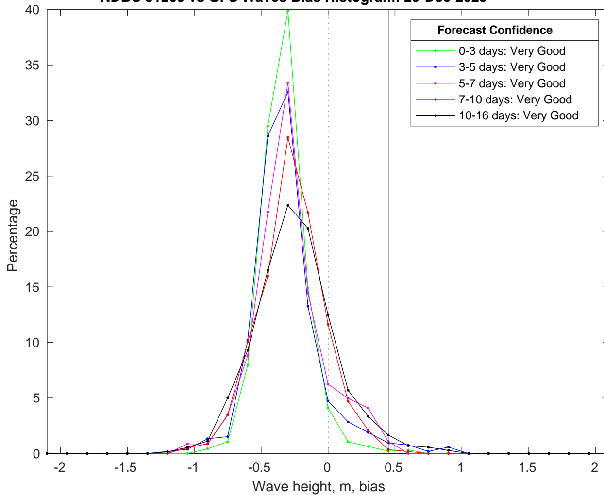
NDBC 51209 vs GFS Waves Bias Histogram: 29-Dec-2025
