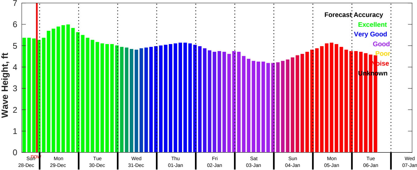
CMEMS Wave Forecast for NDBC 51209 from 28-Dec-2025 13:00:00 to 07-Jan-2026 13:00:00
