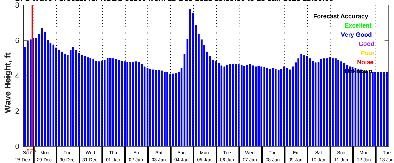
GFS Wave Forecast for NDBC 51209 from 28-Dec-2025 13:00:00 to 13-Jan-2026 13:00:00
