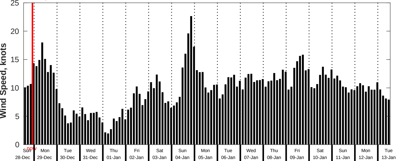
GFS Wind Speed Forecast for NDBC 51209 from 28-Dec-2025 13:00:00 to 13-Jan-2026 13:00:00
