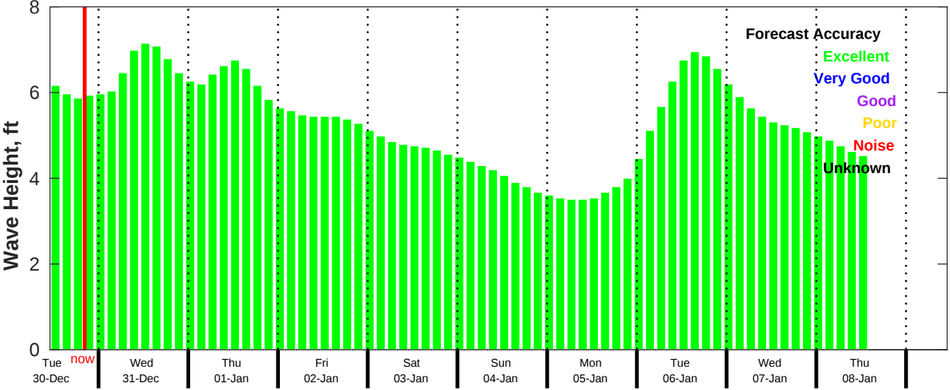
CMEMS Wave Forecast for NDBC 52211 from 29-Dec-2025 11:00:00 to 08-Jan-2026 11:00:00
